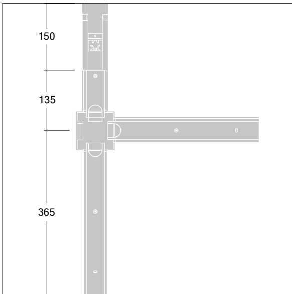
TL_CONTUS_M_T3_Node_Connector.wmf
