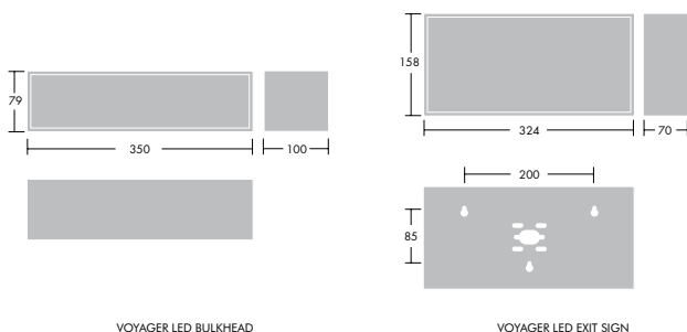
VOYAGER LED BULKHEAD
